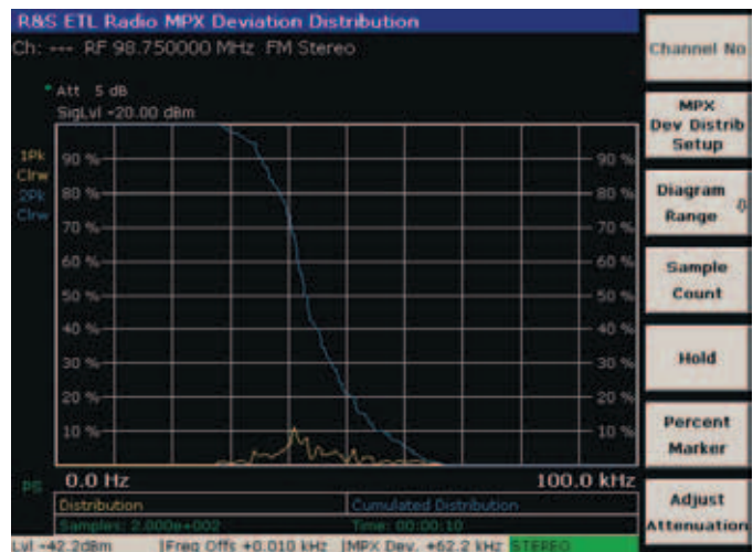
MPX deviation and MPX deviation distribution.
