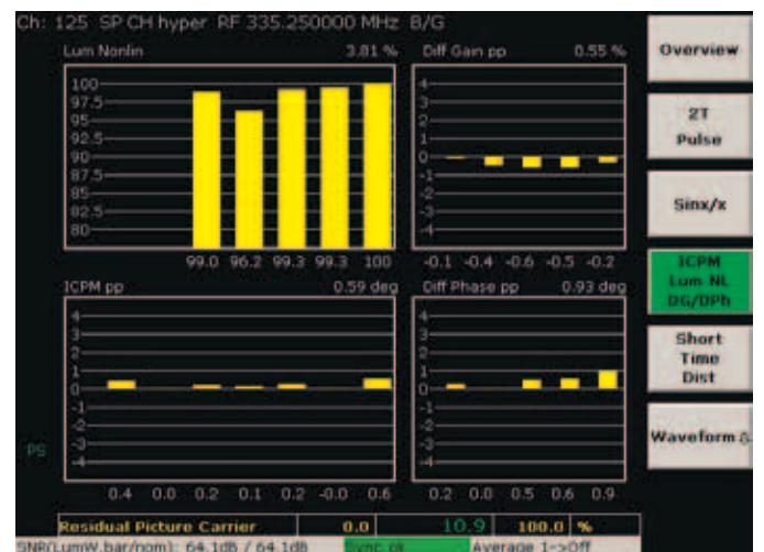
ICPM measurement.
