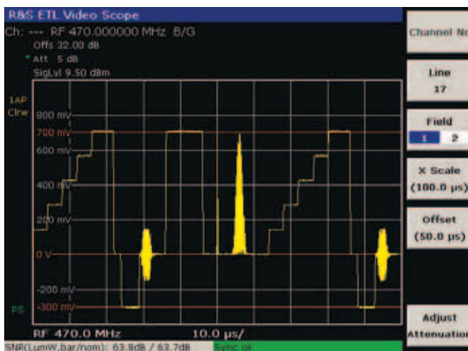
Video line oscilloscope.
