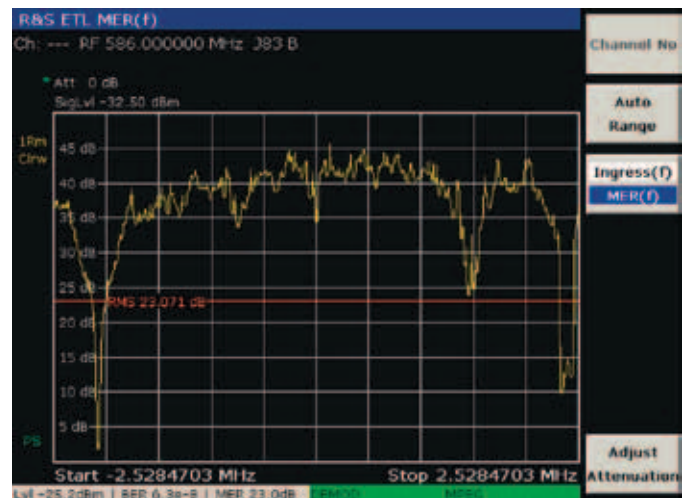
MER (f) of a J.83/B-signal with superimposed interfering.
