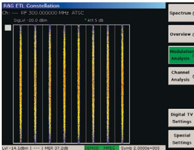
Constellation diagram of an ATSC/8VSB signal.
