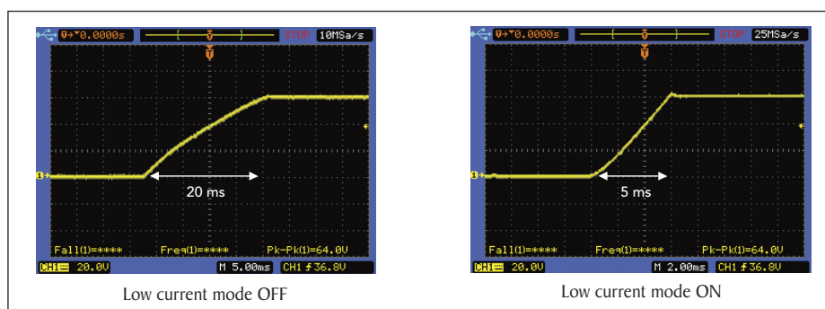
Voltage rise time with and without low current mode enabled
