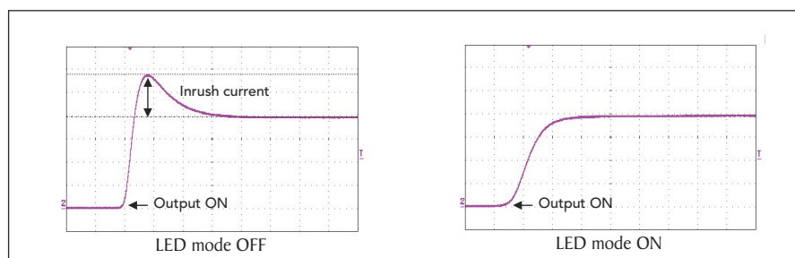
Current flow during power up with LED mode enabled
