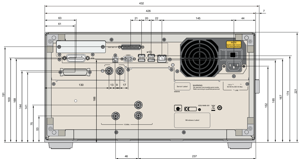
Figure 22. Dimensions (rear view, in millimeters)
